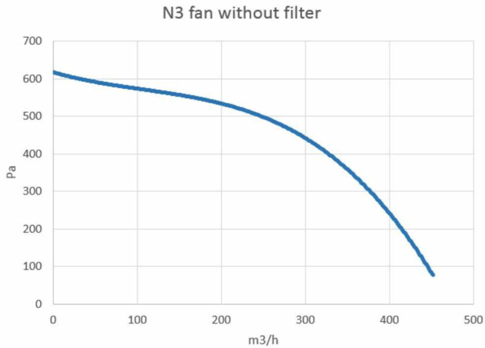
Pressure diagram
